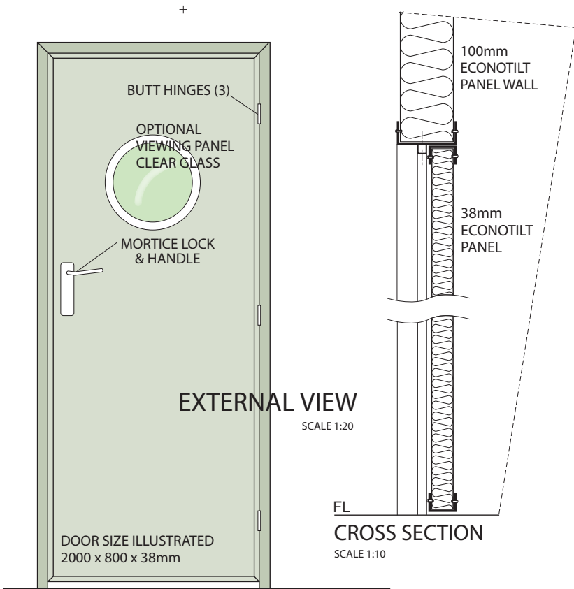
STANDARD OFFICE-TYPE DOOR
