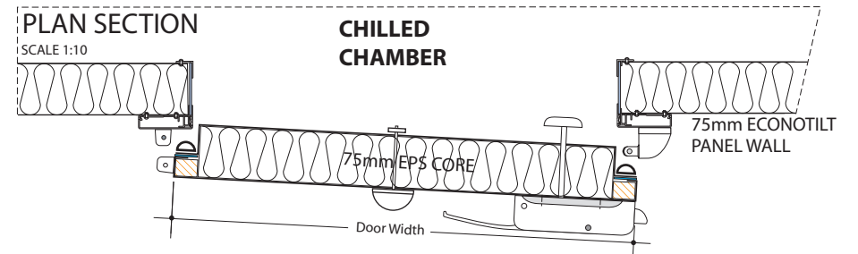
SEMI-FLUSH COOLROOM DOOR WITH INTEGRATED FRAME
