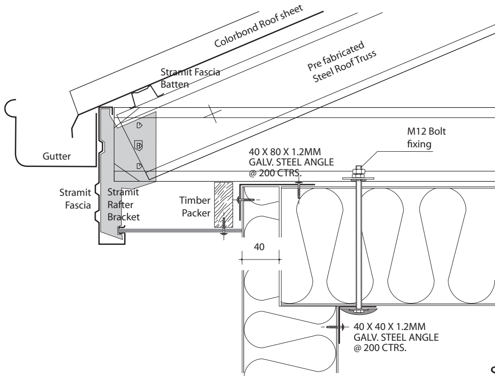
OPTION 1 WITH EAVES
