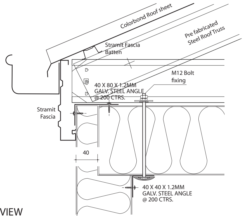
OPTION 2 WITHOUT EAVES
