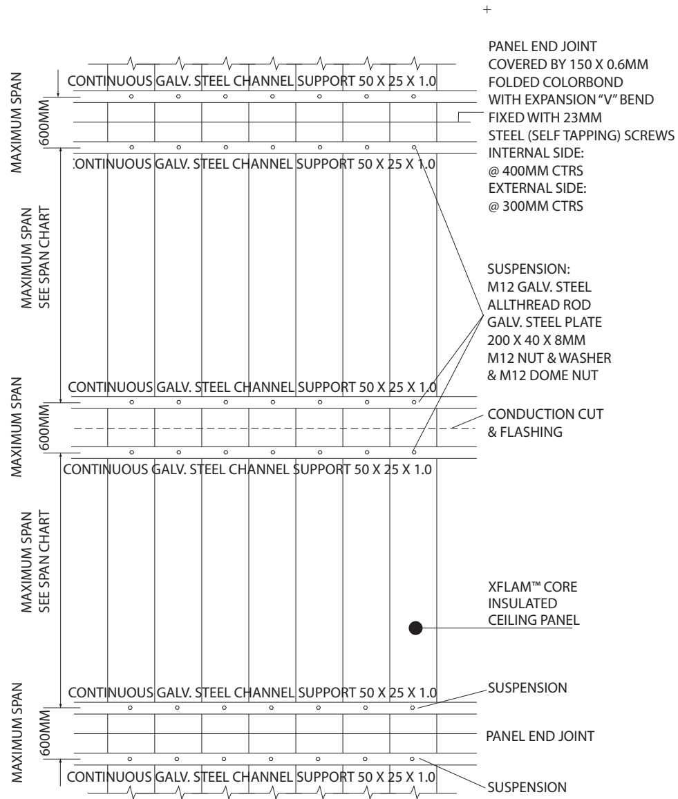
OPTIONAL SUSPENSION PLAN LAYOUT
