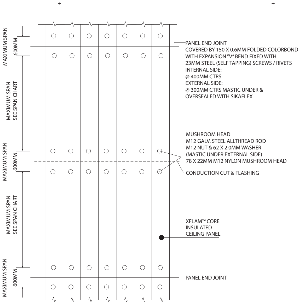
PLAN LAYOUT
