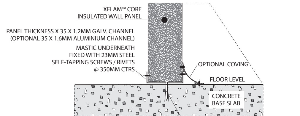
INTERNAL COOLROOM PARTITION WALL
