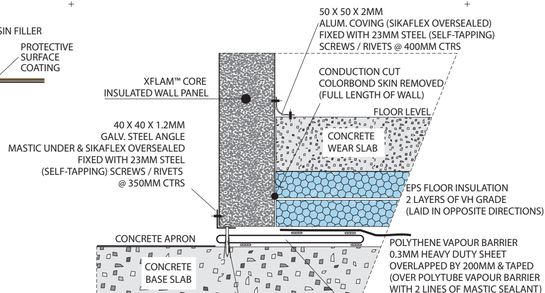
FREEZER WALL BASE
