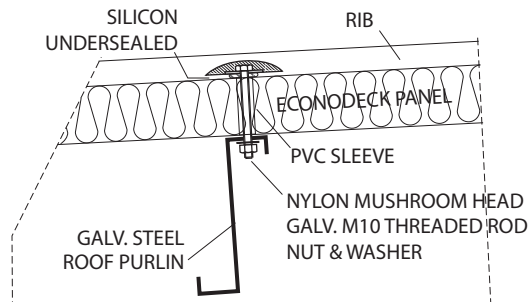
OPTIONAL ROOF FIXING
