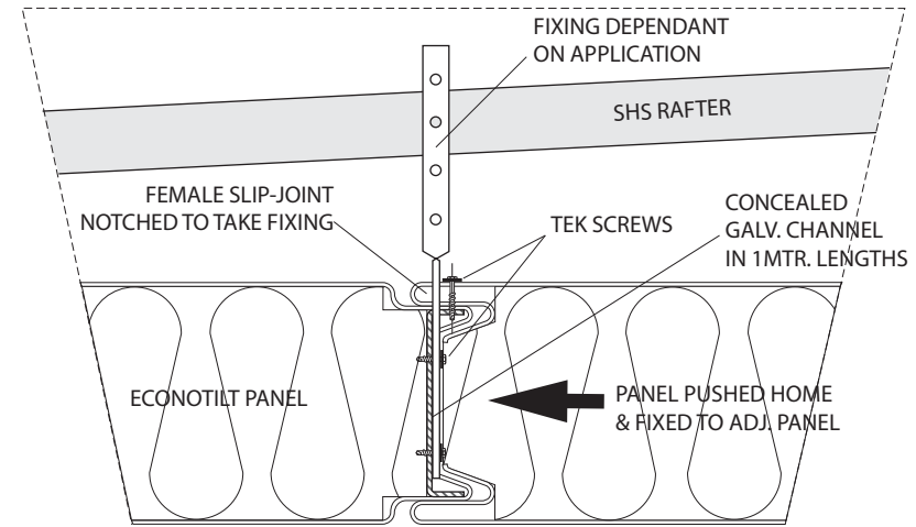
CONCEALED CEILING SUSPENSION
