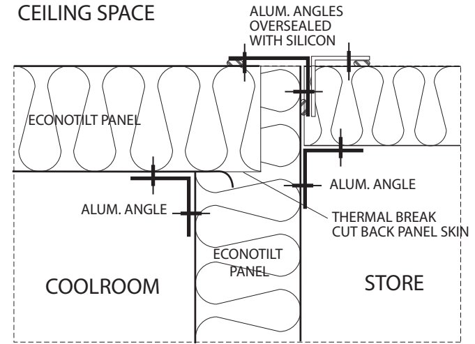
WALL TO CEILING - SECTION
