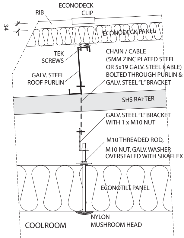
CEILING SUSPENSION - SECTION
